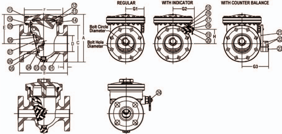
FOR SIZES 3/4" AND 1" ONLY
